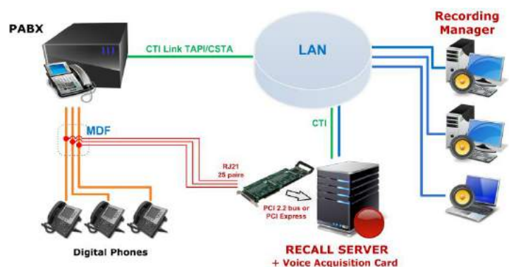
Voice capturing cards in PCI slots for 8, 16 or 24 ports 21x25 pair female D type connector to MDF
